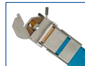
Removable Titanium clamping cassette for UHP 500-2
